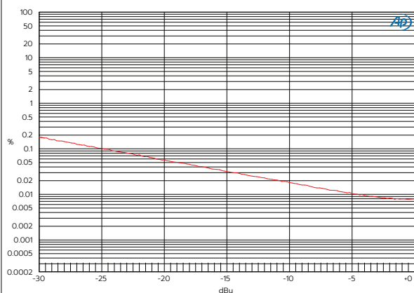
THD+N VS OUTPUT
