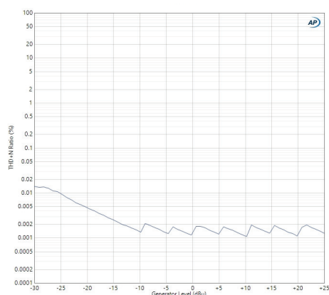
THD+N VS LEVEL
